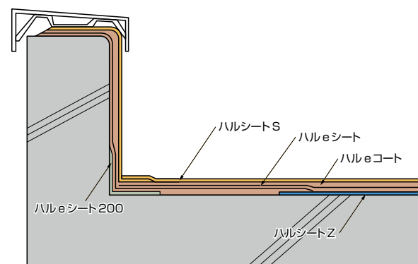
絶縁工法/EZ-30(D-1)
